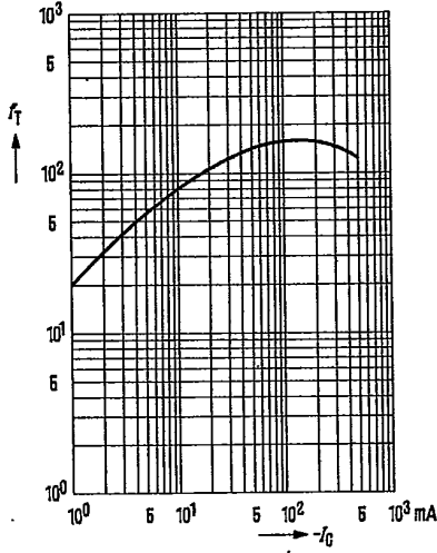
Transition frequency f_T = f(I_C) -V_{CE} = 10 \text{ V} BD 136, BD 138, BD 140
